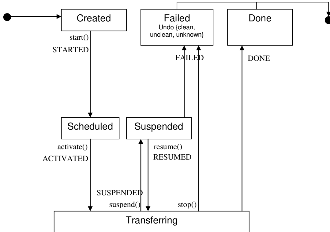
Figure 4: DTI state diagram showing operations() and EVENTS
