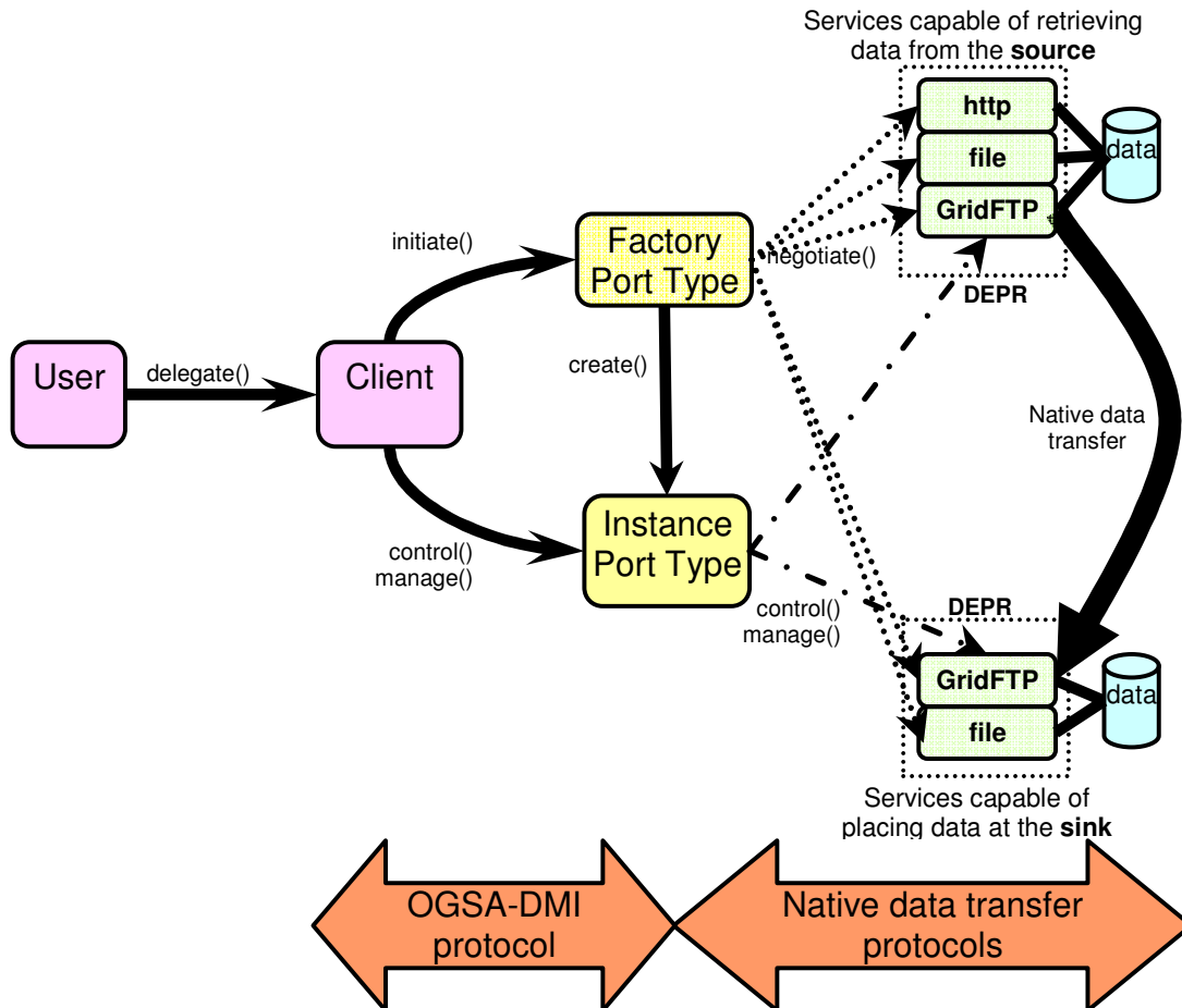
Figure 1: OGSA-DMI Architecture
