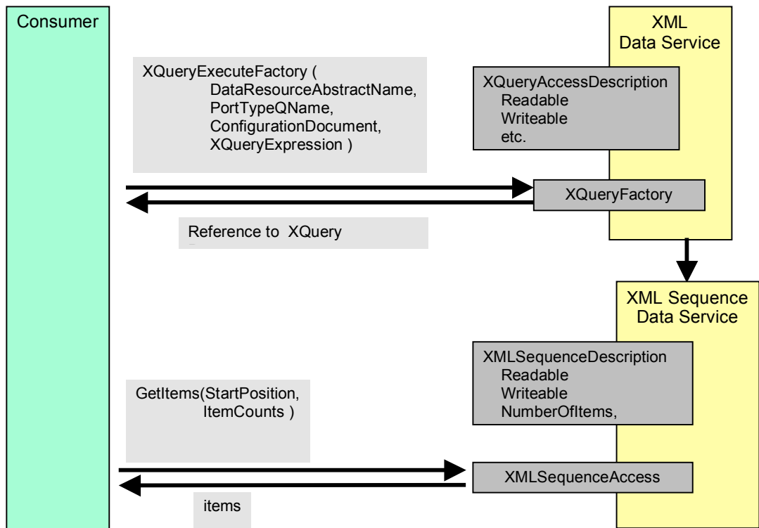
Figure 3: Overview – XQueryFactory
