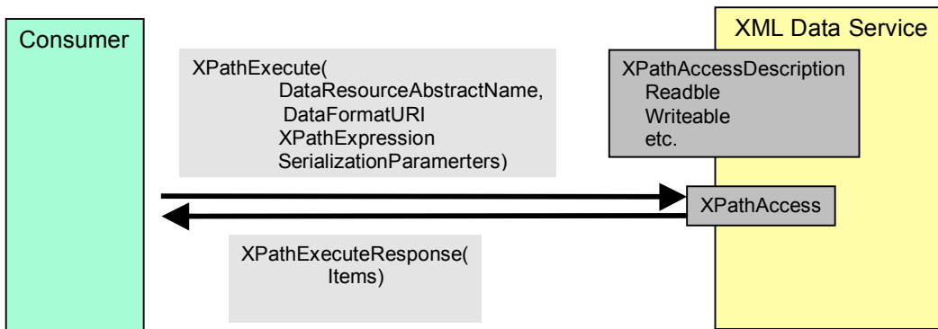
Figure 4: Overview – XPathAccess
