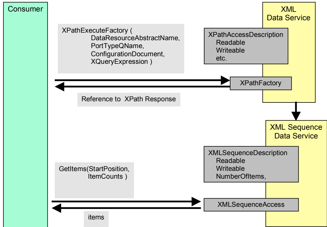
Figure 5: Overview – XPathFactory
