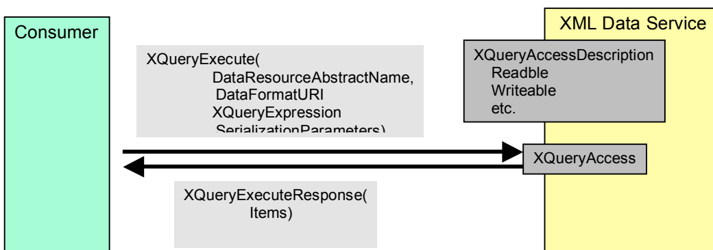
Figure 2: Overview – XQueryAccess
