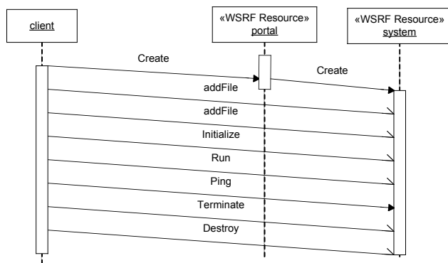
Figure 4 . Sequence diagram of a simple deployment
