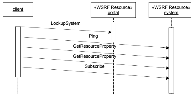
Figure 5. Subscription sequence diagram
